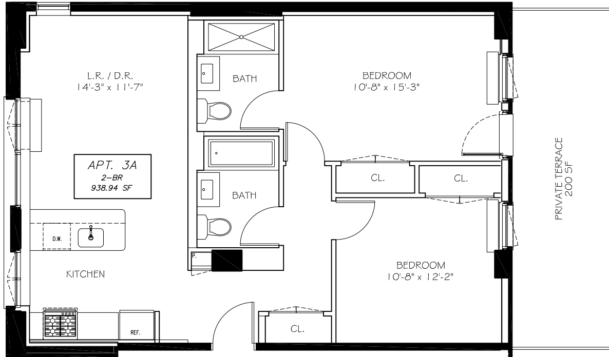
3RD FLOOR PLAN SCALE: 1/4" = 1'-0"
